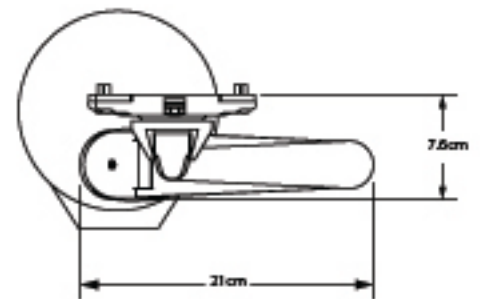
TOP VIEW Arm Folded
