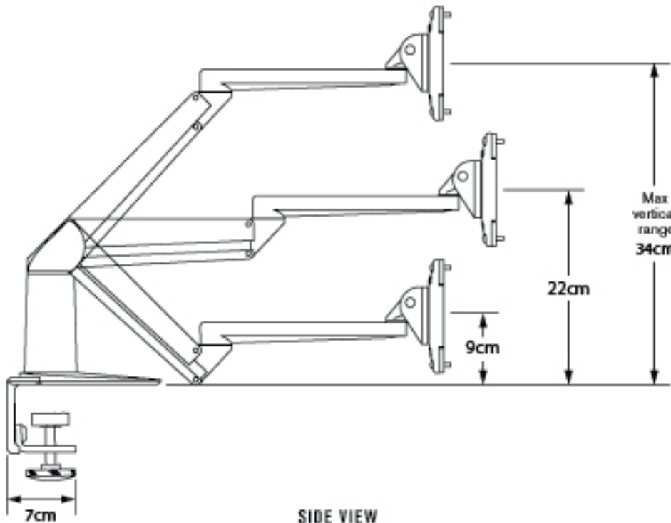
SIDE VIEW Vertical Range
